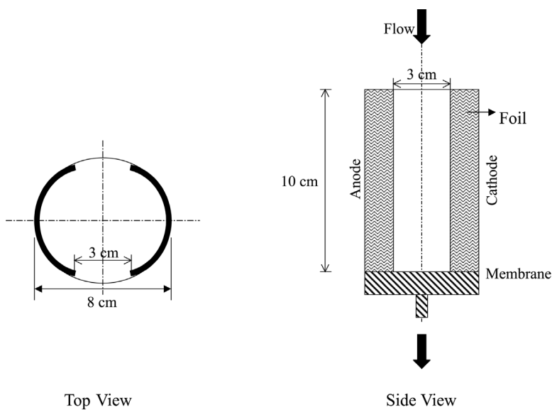
Figure 3. Foil electrode configuration.
